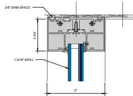
② STANDARD HEAD WITH STRAP ANCHOR 6" = 1'-0"
