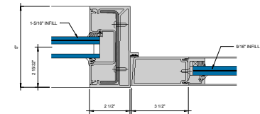
ENTRANCE - 2.75" DOOR JAMB - SINGLE ACTING WITH OFFSET PIVOT OR BUTT HINGE ③ HINGE b" = 1'-0"
