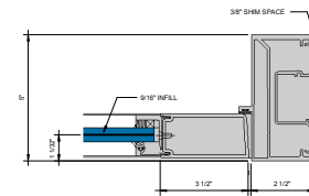
ENTRANCE - DOOR JAMB SINGLE ACTING WITH OFFSET PIVOT OR BUTT HINGE ① 6" = 1'-0"
