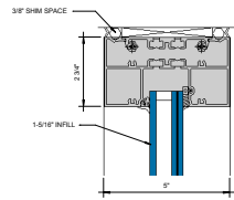
① STANDARD HEAD 6" = 1'-0"
