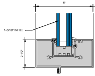
① 1 PIECE HEADER OR TRANSOM BAR WITH INFILL 9" = 1'-0"
