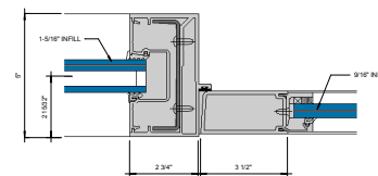
ENTRANCE - 2.75' DOOR JAMB SINGLE ACTING WITH OFFSET PIVOT OR BUTT HINGE ⑦ 6" = 1'-0"
