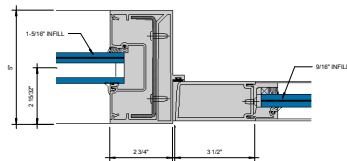
ENTRANCE - 2.75" DOOR JAMB - SINGLE ACTING WITH OFFSET PIVOT OR BUTT HINGE ④ HINGE b" = 1'-0"
