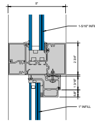
② HEAD AT HORIZONTAL OUTSWING CASEMENT 6" = 1'-0"
