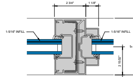
ENTRANCE - 2.75' DOOR JAMB AT TRANSOM AREA WITH SIDELITE OR POCKET INSERT ② 6" = 1'-0"
