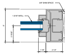
ENTRANCE - DOOR JAMB AT TRANSOM AREA WITH POCKET INSERT ① 6" = 1'-0"
