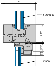
① HEAD AT HORIZONTAL PROJECT-OUT 6" = 1'-0"
