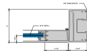
ENTRANCE - 2.75' DOOR JAMB - SINGLE ACTING WITH OFFSET PIVOT OR BUTT HINGE ⑧ 6" = 1'-0"
