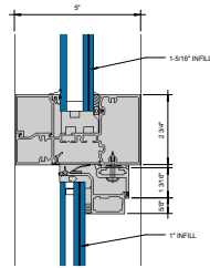
① HEAD AT HORIZONTAL PROJECT-OUT 6" = 1'-0"
