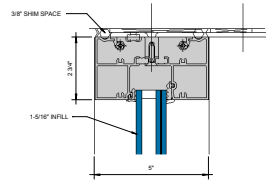
② STANDARD HEAD WITH STRAP ANCHOR 6" = 1'-0"
