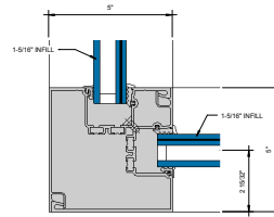
① OUTSIDE 90° CORNER 6" = 1'-0"
