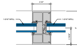
⑩ 2-PIECE VERTICAL 6" = 1'-0"
