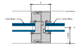
⑪ EXPANSION MULLION 6" = 1'-0"
