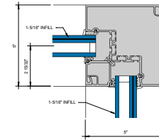
② INSIDE 90° CORNER 6" = 1'-0"
