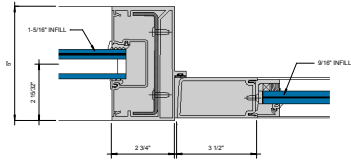
ENTRANCE - 2 7/8\"/>
