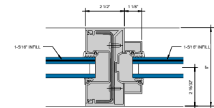
ENTRANCE - DOOR JAMB AT TRANSOM AREA WITH SIDELITE OR POCKET ⑧ INSERT 6" = 1'-0"
