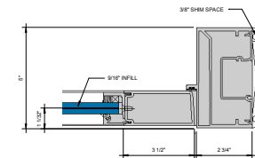
ENTRANCE - 2.75" DOOR JAMB - SINGLE ACTING WITH OFFSET PIVOT OR BUTT HINGE ⑧ HINGE b" = 1'-0"
