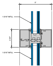
⑤ HORIZONTAL 6" = 1'-0"
