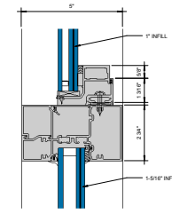
③ SILL AT HORIZONTAL 6" = 1'-0"
