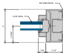
ENTRANCE - DOOR JAMB AT TRANSOM AREA WITH POCKET INSERT ⑩ AREA WITH POCKET INSERT 6" = 1'-0"
