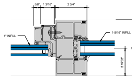
⑤ JAMB AT 3 PIECE VERTICAL MULLION (DEEP POCKET SIDE) 6" = 1'-0"
