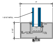
2 PIECE HEADER OR TRANSOM BAR 5" x 1 1/2"
