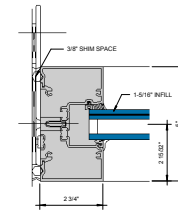
④ OPTIONAL HEAD WITH STRAP ANCHOR 6" = 1'-0"
