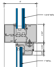
② HEAD AT HORIZONTAL OUTSWING CASEMENT 6" = 1'-0"
