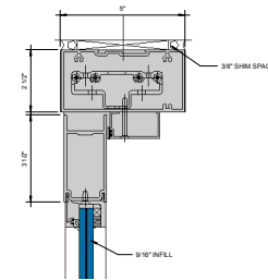
③ COC HEADER BUTT HINGE 6" = 1'-0"
