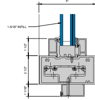
HW COC TRANSOM BAR BUTT HINGE 6" = 1'-0"
