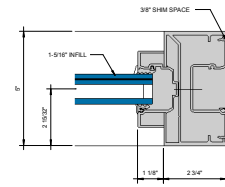
ENTRANCE - 2.75' DOOR JAMB AT TRANSOM AREA WITH POCKET INSERT ③ 6" = 1'-0"
