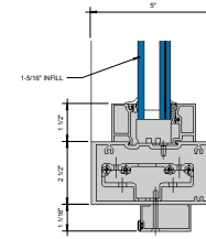
HW GOC TRANSOM BAR BUTT HINGE 5" x 1 1/2"
