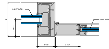
ENTRANCE - DOOR JAMB SINGLE ACTING WITH OFFSET PIVOT OR BUTT HINGE ④ 6" = 1'-0"
