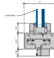
④ HW COC TRANSOM BAR BUTT HINGE 9" = 1'-0"
