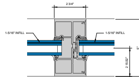
⑩ 2-PIECE VERTICAL 6" = 1'-0"
