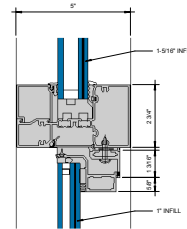
② HEAD AT HORIZONTAL OUTSWING CASEMENT 6" = 1'-0"
