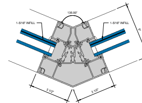
④ OUTSIDE 135° CORNER 6" = 1'-0"
