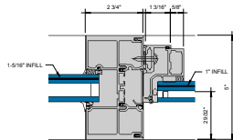
④ JAMB AT 3 PIECE VERTICAL MULLION (SHALLOW POCKET SIDE) 6" = 1'-0"
