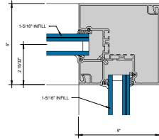
① INSIDE 90° CORNER 6" = 1'-0"
