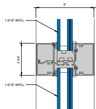
⑤ HORIZONTAL 6" = 1'-0"
