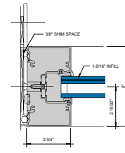
⑧ JAMB WITH STRAP ANCHOR 6" = 1'-0"
