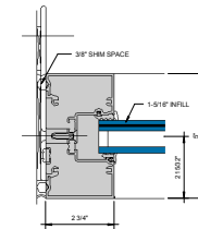
⑧ JAMB WITH STRAP ANCHOR 6" = 1'-0"
