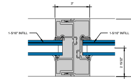
⑪ EXPANSION MULLION 6" = 1'-0"
