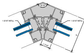
③ INSIDE 135° CORNER 6" = 1'-0"
