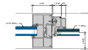
JAMB AT 2 PIECE VERTICAL MULLION ⑥ (SHALLOW POCKET SIDE) 6" = 1'-0"
