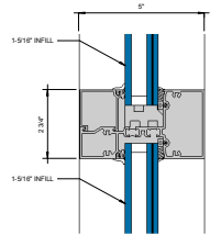
⑤ HORIZONTAL 6" = 1'-0"
