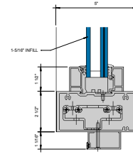
③ HW COC TRANSOM BAR OFFSET PIVOT 9" = 1'-0"
