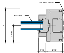
ENTRANCE - DOOR JAMB AT TRANSOM AREA WITH POCKET INSERT ② HINGE b" = 1'-0"
