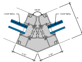
③ OUTSIDE 135° CORNER 6" = 1'-0"
