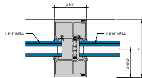
⑨ 3-PIECE VERTICAL 6" = 1'-0"
