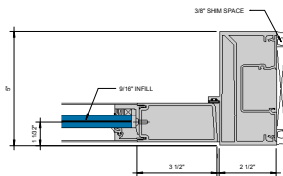
ENTRANCE - MEETING STILE ⑤ 6" = 1'-0"
