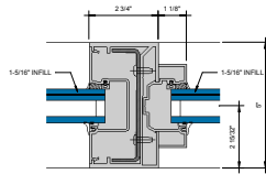
ENTRANCE - 2.75" DOOR JAMB AT TRANSOM AREA WITH SIDELITE OR POCKET INSERT ① HINGE b" = 1'-0"
