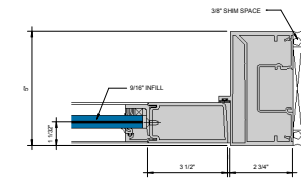
ENTRANCE - 2.75" DOOR JAMB - SINGLE ACTING WITH OFFSET PIVOT OR BUTT HINGE ② 6" = 1'-0"
