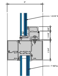
③ SILL AT HORIZONTAL 6" = 1'-0"
