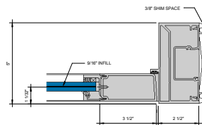
ENTRANCE - DOOR JAMB SINGLE ACTING WITH OFFSET PIVOT OR BUTT HINGE ⑥ 6" = 1'-0"
