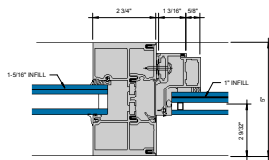
JAMB AT 3 PIECE VERTICAL MULLION ④ (SHALLOW POCKET SIDE) 6" = 1'-0"
