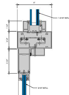
⑥ COC TRANSOM BAR BUTT HINGE 6" = 1'-0"
