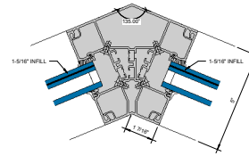
② INSIDE 135° CORNER 6" = 1'-0"
