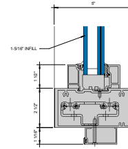
HW GOC TRANSOM BAR OFFSET PIVOT 5" x 1 1/2"
