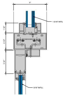
⑥ COC TRANSOM BAR BUTT HINGE 6" = 1'-0"
