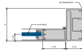
ENTRANCE - DOOR JAMB SINGLE ACTING WITH OFFSET PIVOT OR BUTT HINGE \phi = 1.0"
