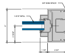
ENTRANCE - 2.75" DOOR JAMB AT TRANSOM AREA WITH POCKET INSERT ⑪ TRANSOM AREA WITH POCKET INSERT 6" = 1'-0"
