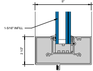
1 PIECE HEADER OR TRANSOM BAR WITH FIN 6" = 1'-0"
