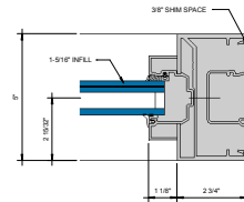
ENTRANCE - 2.75" DOOR JAMB AT TRANSOM AREA WITH POCKET INSERT ① HINGE b" = 1'-0"
