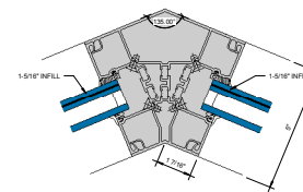
④ INSIDE 135° CORNER 6" = 1'-0"
