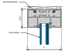
① STANDARD HEAD 6" = 1'-0"
