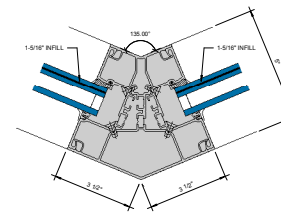
④ OUTSIDE 135° CORNER 6" = 1'-0"
