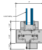
⑦ COC TRANSOM BAR BUTT HINGE 9" = 1'-0"
