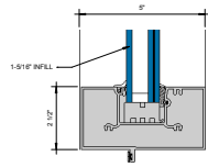
1 PIECE HEADER OR TRANSOM BAR WITH FIN 5" x 1 1/2"
