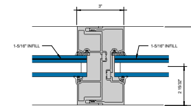
⑪ EXPANSION MULLION 6" = 1'-0"
