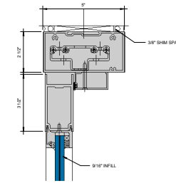
③ COC HEADER BUTT HINGE 6" = 1'-0"
