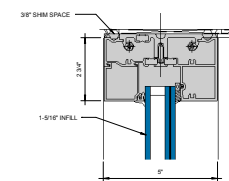
④ OPTIONAL HEAD WITH STRAP ANCHOR 6" = 1'-0"
