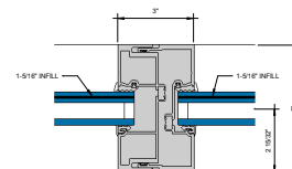
⑪ EXPANSION MULLION 6" = 1'-0"
