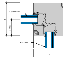
② INSIDE 90° CORNER 6" = 1'-0"
