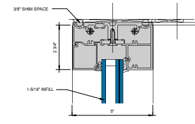
④ OPTIONAL HEAD WITH STRAP ANCHOR 6" = 1'-0"
