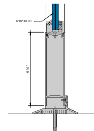
⑦ BOTTOM RAIL 6" = 1'-0"
