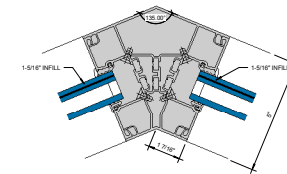
④ INSIDE 135° CORNER 6" = 1'-0"
