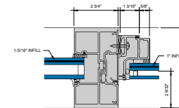
⑥ JAMB AT 2 PIECE VERTICAL MULLION (SHALLOW POCKET SIDE) 6" = 1'-0"
