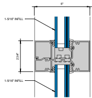
⑤ HORIZONTAL 6" = 1'-0"
