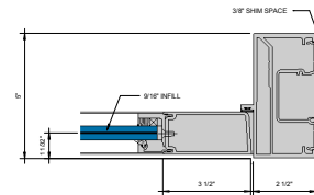
ENTRANCE - 2.75" DOOR JAMB SINGLE ACTING WITH OFFSET PIVOT OR BUTT HINGE ⑦ HINGE b" = 1'-0"
