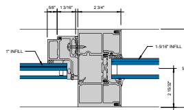
JAMB AT 3 PIECE VERTICAL MULLION ⑤ (DEEP POCKET SIDE) 6" = 1'-0"
