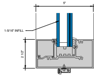
2 PIECE HEADER OR TRANSOM BAR 6" = 1'-0"
