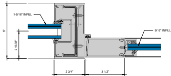
ENTRANCE - 2.75" DOOR JAMB - SINGLE ACTING WITH OFFSET PIVOT OR BUTT HINGE ① 6" = 1'-0"
