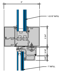
① HEAD AT HORIZONTAL PROJECT OUT 6" = 1'-0"
