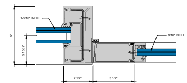
ENTRANCE - DOOR JAMB SINGLE ACTING WITH OFFSET PIVOT OR BUTT HINGE ⑫ HINGE 6" = 1'-0"
