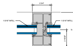
⑩ 2 PIECE VERTICAL 6" = 1'-0"
