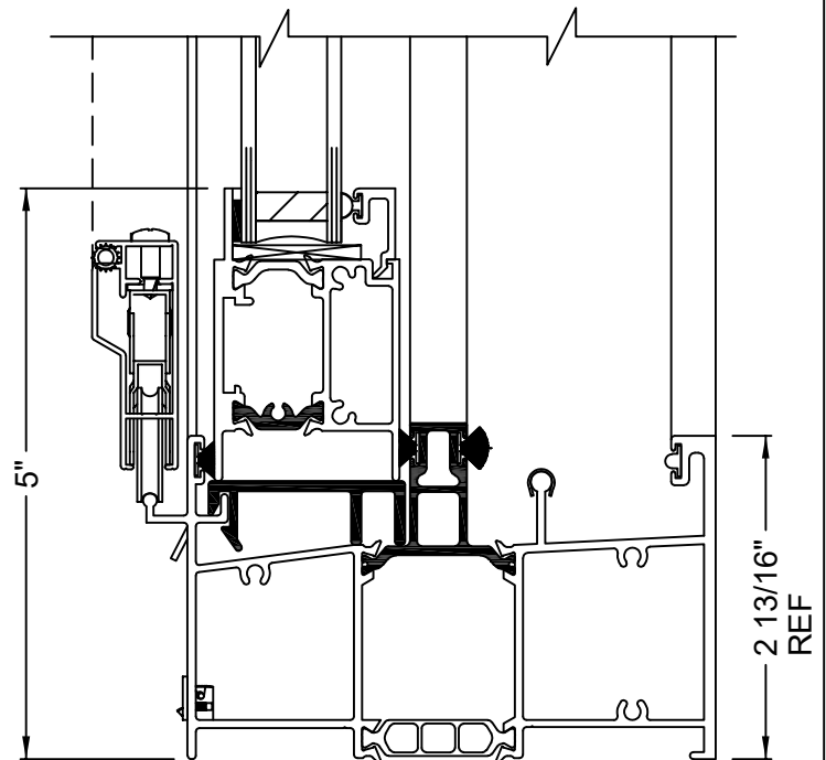
④ FIXED SILL
