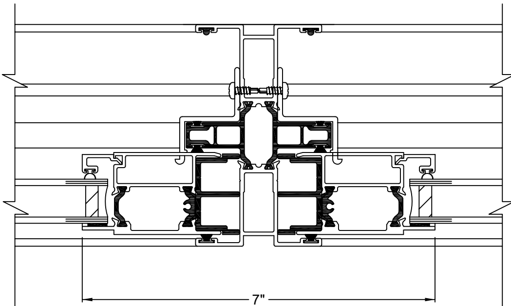
⑨ FIXED INTERMEDIATE MULLION
