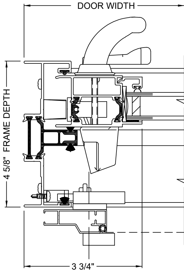
⑤ OPERATING JAMB
