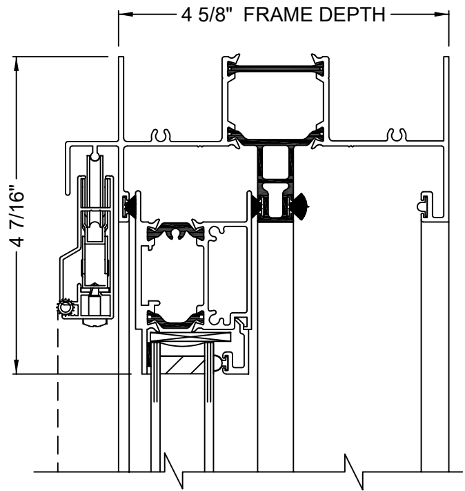
③ FIXED HEAD
