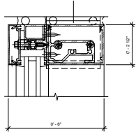
① Curtain Wall Mullion-Head-Kawneer-1600UT-System1-Double Glass-6" 6" = 1'-0"
