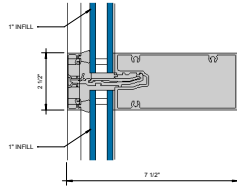
② HORIZONTAL - 1" INFILL 6" = 1'-0"
