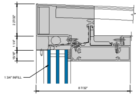
① HEAD - 1-3/4" INFILL 6" = 1'-0"
