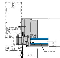
⑥ LEFT JAMB COS- 1" INFILL 6" = 1"
