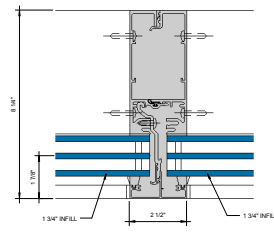
⑥ VERTICAL MULLION - 1-3/4" INFILL 6" = 1'-0"
