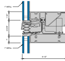
③ SGT EXPANSION HORIZONTAL - 1" INFILL 6" = 1'-0"
