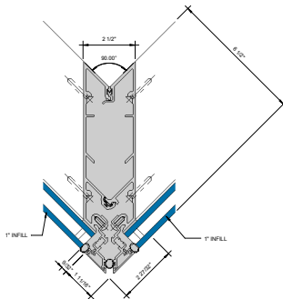
⑧ SGT 90° OUTSIDE CORNER - 1" INFILL 6" = 1'-0"
