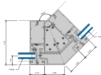
⑩ 135° OUTSIDE CORNER - 1" INFILL 6" = 1'-0"
