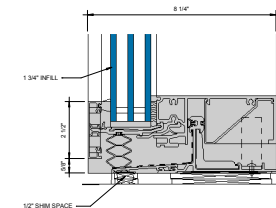
④ SILL - 1-3/4" INFILL 6" = 1'-0"
