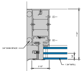
⑤ SGT JAMB - 1-3/4" INFILL Ø = 1'-0"
