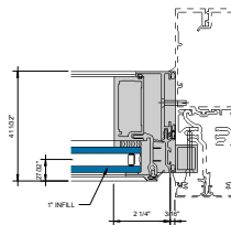
⑤ RIGHT JAMB PO- 1" INFILL 6" = 1"
