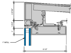
① SGT HEAD - 1" INFILL 6" = 1'-0"
