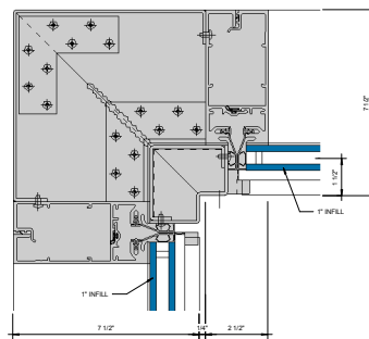
⑨ 90° INSIDE CORNER - 1" INFILL 6" x 1'-0"
