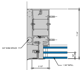
⑤ SGT JAMB - 1-3/4" INFILL 6" = 1'-0"
