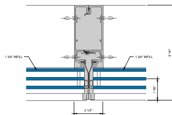
⑥ SGT VERTICAL MULLION - 1-3/4" INFILL 6" = 1'-0"
