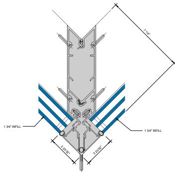
⑧ 90° OUTSIDE CORNER - 1-3/4" INFILL 6" = 1'-0"
