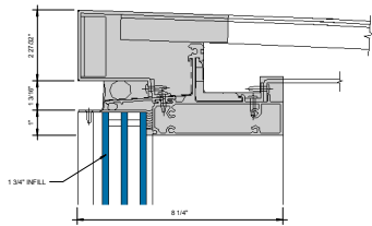
① HEAD - 1-3/4" INFILL 6" = 1'-0"
