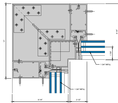
⑨ 90° INSIDE CORNER - 1-3/4" INFILL 6" = 1'-0"
