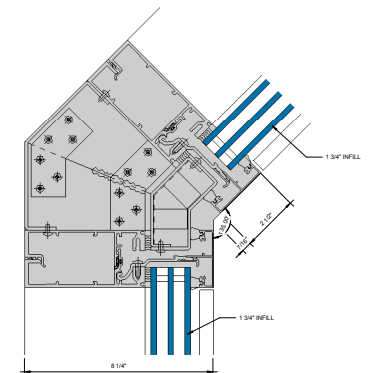
⑪ 135° INSIDE CORNER - 1-3/4" INFILL 6" = 1'-0"
