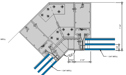
⑪ SGT 135° INSIDE CORNER - 1-3/4" INFILL 6" = 1'-0"
