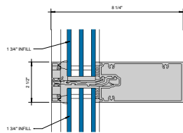
② HORIZONTAL - 1-3/4" INFILL 6" = 1'-0"
