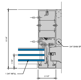
⑦ JAMB - 1-3/4" INFILL 6" = 1'-0"
