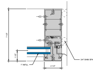
⑦ JAMB - 1" INFILL 6" = 1'-0"
