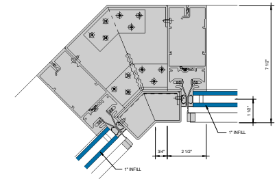
⑪ 135° INSIDE CORNER - 1" INFILL 6" x 1'-0"
