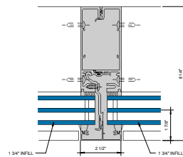
⑥ VERTICAL MULLION - 1-3/4" INFILL 6" = 1'-0"
