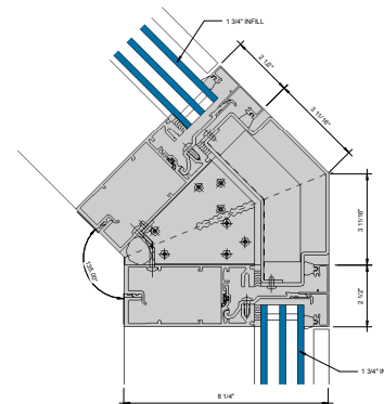
⑩ 135° OUTSIDE CORNER - 1-3/4" INFILL 6" = 1'-0"
