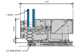
④ SILL - 1" INFILL 6" = 1'-0"
