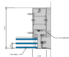
⑦ SGT JAMB - 1-3/4" INFILL 6" = 1'-0"
