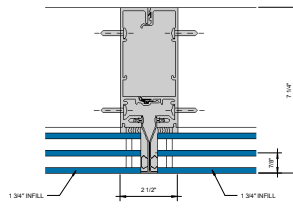
⑥ SGT VERTICAL MULLION - 1-3/4" INFILL 6" = 1'-0"
