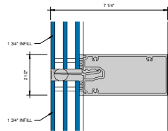
② SGT HORIZONTAL - 1-3/4" INFILL Ø = 1'-0"
