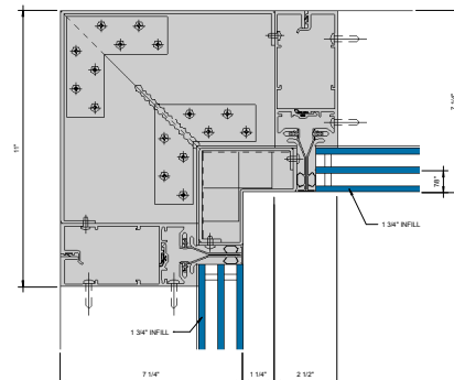
⑨ SGT 90° INSIDE CORNER - 1-3/4" INFILL 6" = 1'-0"
