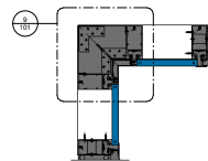
④ SGT 90° INSIDE CORNER 1 1/2" x 1'-0"
