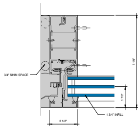
⑤ JAMB - 1-3/4" INFILL 6" = 1'-0"
