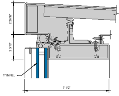
① HEAD - 1" INFILL 6" = 1'-0"
