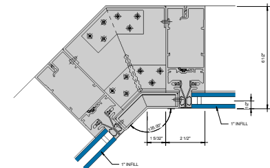
⑪ SGT 135° INSIDE CORNER - 1" INFILL 6" = 1'-0"
