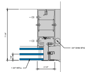
⑦ SGT JAMB - 1-3/4" INFILL Ø = 1'-0"
