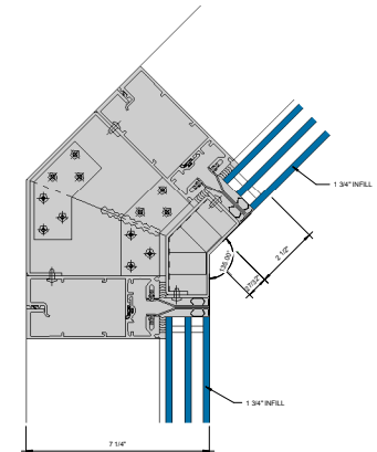
⑪ SGT 135° INSIDE CORNER - 1-3/4" INFILL Ø = 1'-0"
