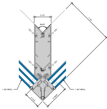
⑧ SGT 90° OUTSIDE CORNER - 1-3/4" INFILL 6" = 1'-0"
