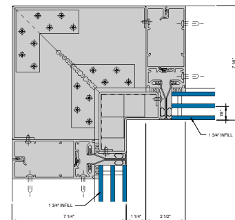
⑨ SGT 90° INSIDE CORNER - 1-3/4" INFILL Ø = 1'-0"
