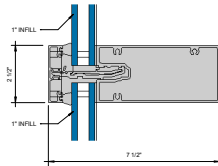
② HORIZONTAL - 1" INFILL 6" x 1'-0"
