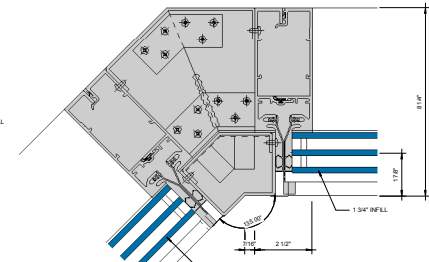
⑪ 135° INSIDE CORNER - 1-3/4" INFILL 6" = 1'-0"
