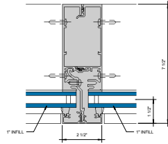
⑥ VERTICAL MULLION - 1" INFILL 6" = 1'-0"
