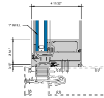
③ SILL- 1" INFILL 6" = 1"
