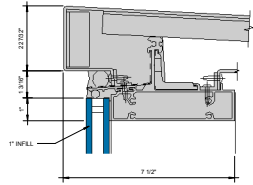
① SGT HEAD - 1" INFILL 6" x 1'-0"
