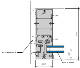
⑤ JAMB - 1" INFILL 6" = 1'-0"
