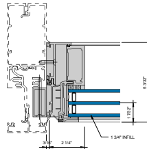
⑤ LEFT JAMB COS - 1-3/4" INFILL 6" = 1'-0"
