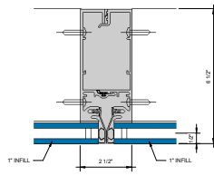
⑥ SGT VERTICAL MULLION - 1" INFILL 6" x 1'-0"
