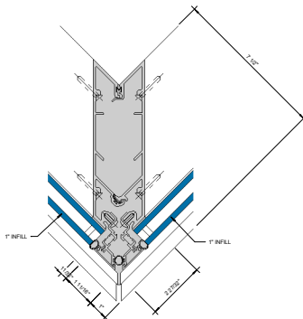
⑧ 90° OUTSIDE CORNER - 1" INFILL 6" x 1'-0"
