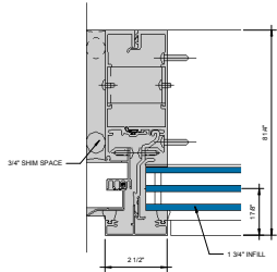
⑤ SGT JAMB - 1-3/4" INFILL 6" = 1'-0"
