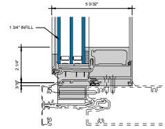
③ SILL - 1-3/4" INFILL 6" = 1'-0"
