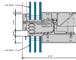
③ EXPANSION HORIZONTAL - 1-3/4" INFILL 6" = 1'-0"
