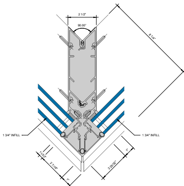
⑧ 90° OUTSIDE CORNER - 1-3/4" INFILL 6" = 1'-0"
