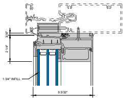
① HEAD PO - 1-3/4" INFILL 6" = 1'-0"
