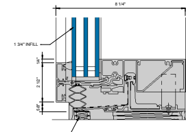
④ SILL - 1-3/4" INFILL 6" = 1'-0"
