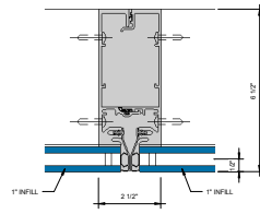
⑥ SGT VERTICAL MULLION - 1" INFILL 6" = 1'-0"
