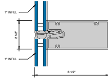
② SGT HORIZONTAL - 1" INFILL 6" = 1'-0"
