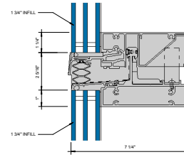
③ SGT EXPANSION HORIZONTAL - 1-3/4" INFILL 6" = 1'-0"
