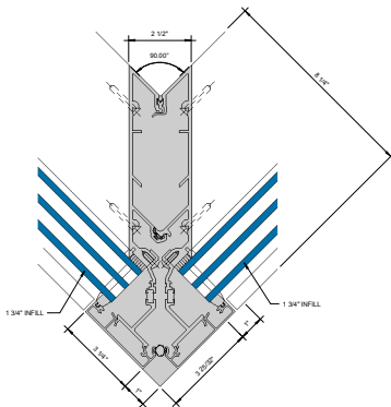
⑧ 90° OUTSIDE CORNER - 1-3/4" INFILL 6" = 1'-0"
