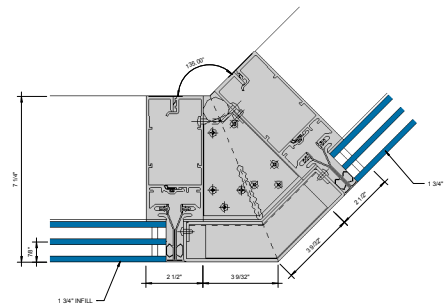
⑩ SGT 135° OUTSIDE CORNER - 1-3/4" INFILL 6" = 1'-0"
