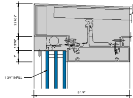
① HEAD - 1-3/4" INFILL 6" = 1'-0"
