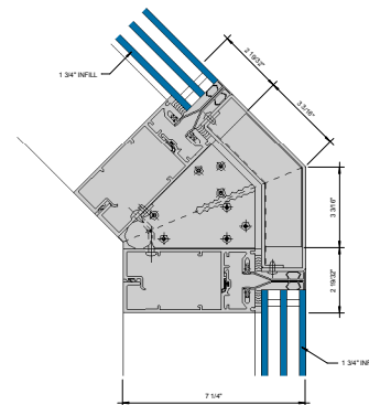
⑩ SGT 135° OUTSIDE CORNER - 1-3/4" INFILL Ø = 1'-0"
