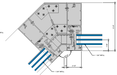
⑪ 135° INSIDE CORNER - 1-3/4" INFILL 6" = 1'-0"
