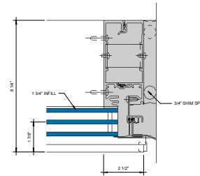
⑦ SGT JAMB - 1-3/4" INFILL 6" = 1'-0"
