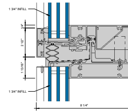
③ EXPANSION HORIZONTAL - 1-3/4" INFILL 6" = 1'-0"
