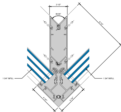
⑧ 90° OUTSIDE CORNER - 1-3/4" INFILL 6" = 1'-0"
