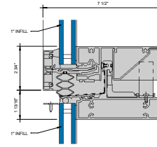
③ EXPANSION HORIZONTAL - 1" INFILL 6" = 1'-0"
