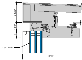
① SGT HEAD - 1-3/4" INFILL 6" = 1'-0"
