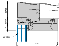
① SGT HEAD - 1-3/4" INFILL Ø = 1'-0"
