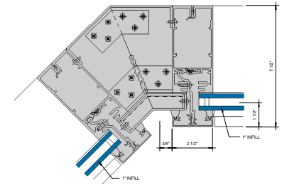
⑪ 135° INSIDE CORNER - 1" INFILL 6" = 1'-0"
