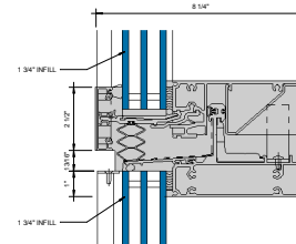
③ EXPANSION HORIZONTAL - 1-3/4" INFILL 6" = 1'-0"
