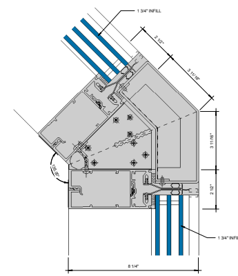
⑩ 135° OUTSIDE CORNER - 1-3/4" INFILL 6" = 1'-0"
