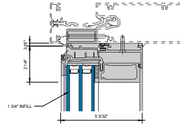
② HEAD COS - 1-3/4" INFILL 6" = 1'-0"
