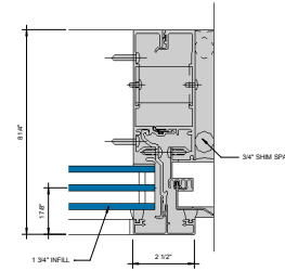
⑦ SGT JAMB - 1-3/4" INFILL 6" = 1'-0"
