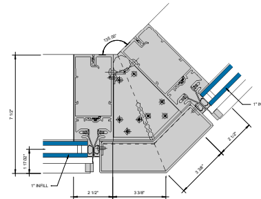
⑩ 135° OUTSIDE CORNER - 1" INFILL 6" x 1'-0"
