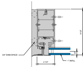
⑤ SGT JAMB - 1" INFILL 6" = 1'-0"
