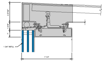
① SGT HEAD - 1-3/4" INFILL 6" = 1'-0"
