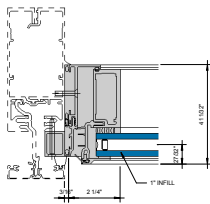
④ LEFT JAMB PO- 1" INFILL 6" = 1"
