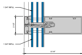
② HORIZONTAL - 1-3/4" INFILL 6" = 1'-0"
