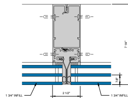
⑥ SGT VERTICAL MULLION - 1-3/4" INFILL Ø = 1'-0"
