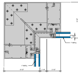
⑨ SGT 90° INSIDE CORNER - 1" INFILL 6" = 1'-0"
