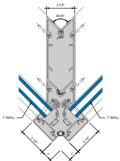
⑧ 90° OUTSIDE CORNER - 1" INFILL 6" = 1'-0"
