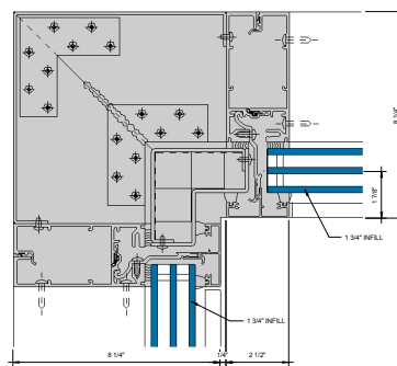
⑨ 90° INSIDE CORNER - 1-3/4" INFILL 6" = 1'-0"
