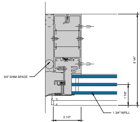
⑤ SGT JAMB - 1-3/4" INFILL 6" = 1'-0"
