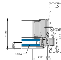
⑦ RIGHT JAMB COS- 1" INFILL 6" = 1"
