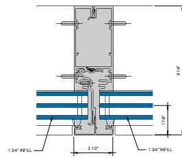
⑥ SGT VERTICAL MULLION - 1-3/4" INFILL 6" = 1'-0"
