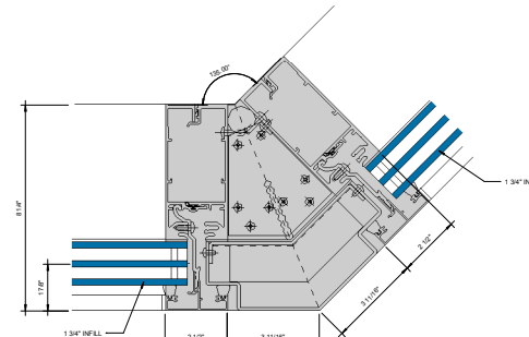
⑩ 135° OUTSIDE CORNER - 1-3/4" INFILL 6" = 1'-0"
