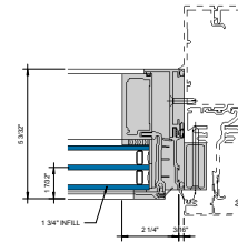
⑦ RIGHT JAMB COS - 1-3/4" INFILL 6" = 1'-0"
