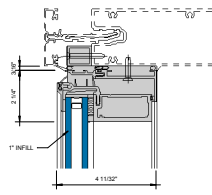
② HEAD COS- 1" INFILL 6" = 1"
