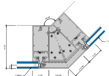
⑩ SGT 135° OUTSIDE CORNER - 1" INFILL 6" = 1'-0"
