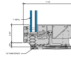
④ SILL - 1" INFILL 6" x 1'-0"
