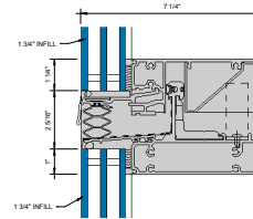
SGT EXPANSION HORIZONTAL - 1-3/4" INFILL Ø = 1'-0"
