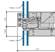
③ EXPANSION HORIZONTAL - 1" INFILL 6" x 1'-0"
