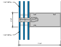
② SGT HORIZONTAL - 1-3/4" INFILL 6" = 1'-0"
