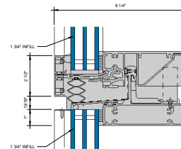
③ EXPANSION HORIZONTAL - 1-3/4" INFILL 6" = 1'-0"
