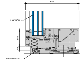
④ SILL - 1-3/4" INFILL 6" = 1'-0"
