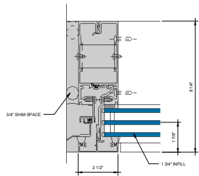
⑤ JAMB - 1-3/4" INFILL 6" = 1'-0"
