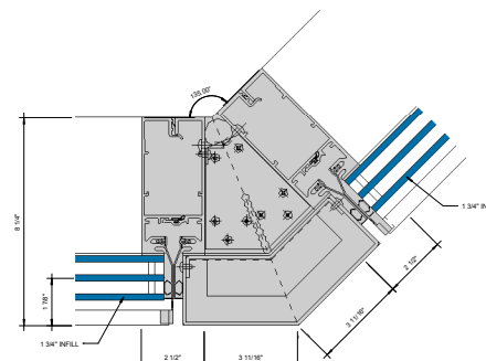
⑩ 135° OUTSIDE CORNER - 1-3/4" INFILL 6" = 1'-0"
