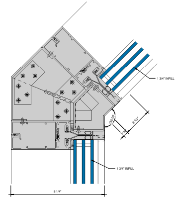
⑪ 135° INSIDE CORNER - 1-3/4" INFILL 6" = 1'-0"
