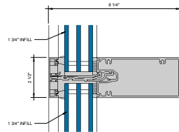
② HORIZONTAL - 1-3/4" INFILL 6" = 1'-0"
