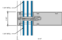
② HORIZONTAL - 1-3/4" INFILL 6" = 1'-0"
