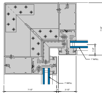
⑨ 90° INSIDE CORNER - 1" INFILL 6" = 1'-0"
