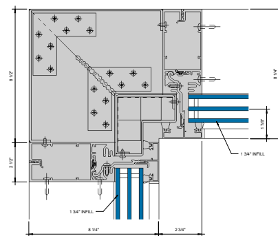
⑨ 90° INSIDE CORNER - 1-3/4" INFILL 6" = 1'-0"
