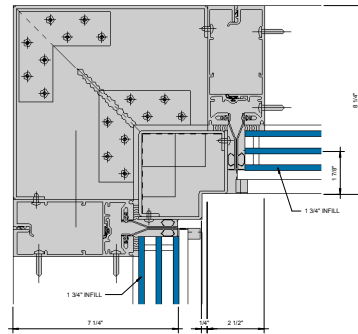
⑨ SGT 90° INSIDE CORNER - 1-3/4" INFILL 6" = 1'-0"
