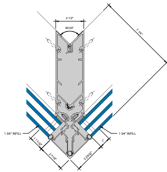
⑧ SGT 90° OUTSIDE CORNER - 1-3/4" INFILL Ø = 1'-0"
