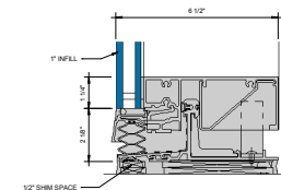
④ SGT SILL - 1" INFILL 6" = 1'-0"
