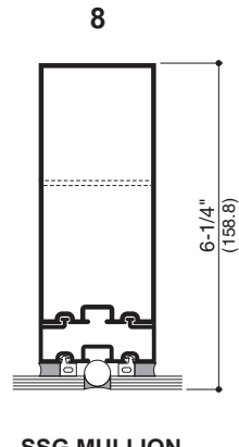
SSG MULLION
