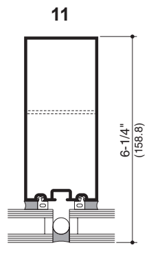
SSG MULLIONS
